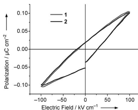
Figure 4. E – P hysteresis loops on thin films of 1 and 2 .
