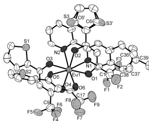
Figure 1. The structure of 1 showing 50% probability displacement ellipsoids; H atoms are omitted for clarity. Selected bond lengths [ \text{\AA} ] and angles [ ^\circ ]: Eu1-O1 2.383(7), Eu1-O2 2.363(6), Eu1-O3 2.357(7), Eu1-O4 2.370(7), Eu1-O5 2.392(7), Eu1-O6 2.355(7), Eu1-N1 2.546(8), Eu1-N2 2.586(8); O1-Eu1-O3 116.1(3), O2-Eu1-O4 119.7(3), O5-Eu1-N1 109.7(3), O6-Eu1-N2 106.9(3).
